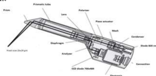
Figure 11. Scheme of Cerec 2 scanner head section
